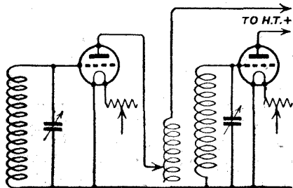
Fig. 5.—A type of coupling similar in effect to that shown in Fig. 4, with tapplings on the primary of the H.F. transformer.
